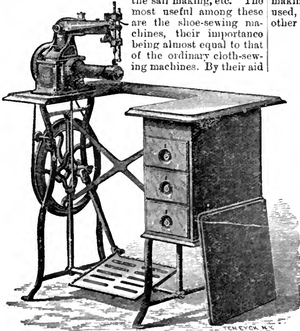
Cylinder Sewing-machine.
