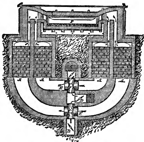
FIG. 3.—Open hearth Furnace.
