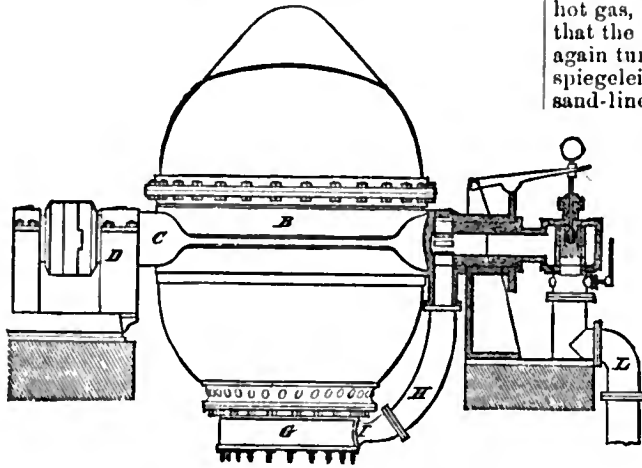
FIG. 1.—Bessemer Converter.
