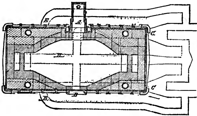
Fig. 6.—Open-hearth Furnace.
