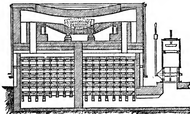
FIG. 5.—Open hearth Furnace.
